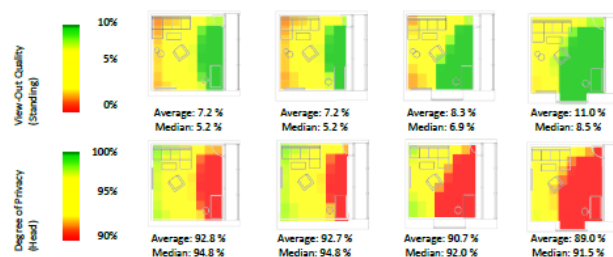
Fig. 1: Simulation output of evaluation metrics. For further details please refer to the full paper.
